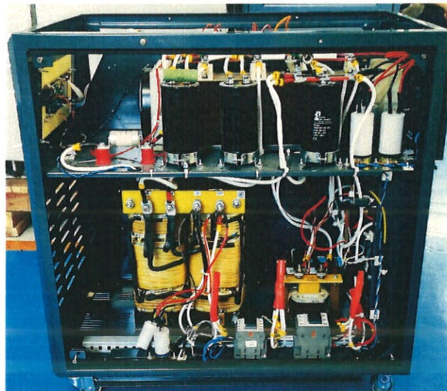
INTERNAL VIEW
